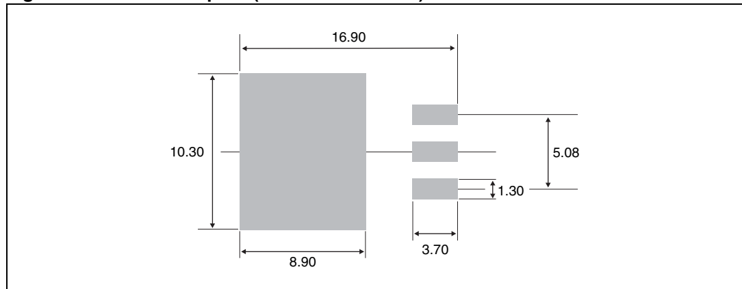
Figure 14. D 2 PAK footprint (dimensions in mm)
