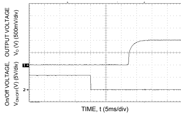
Figure 48. Typical Start-Up Using Remote On/Off, negative logic version shown.
