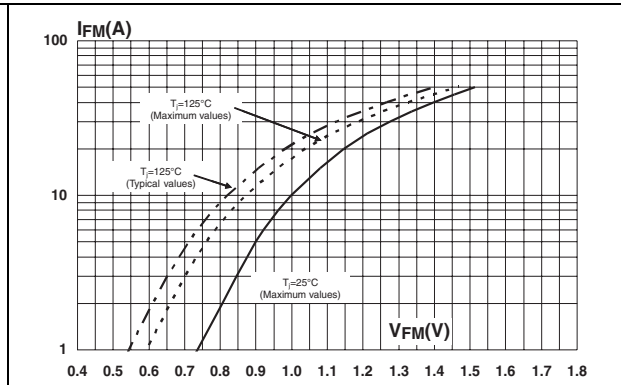
Figure 14. Forward voltage drop versus forward current (high level)
