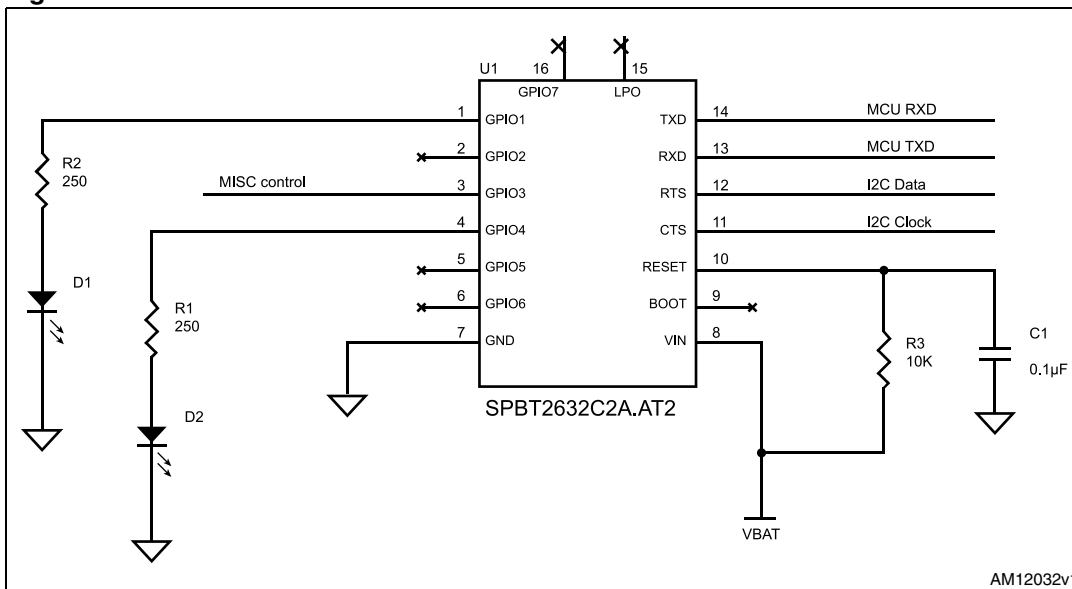
Figure 12. BT module
