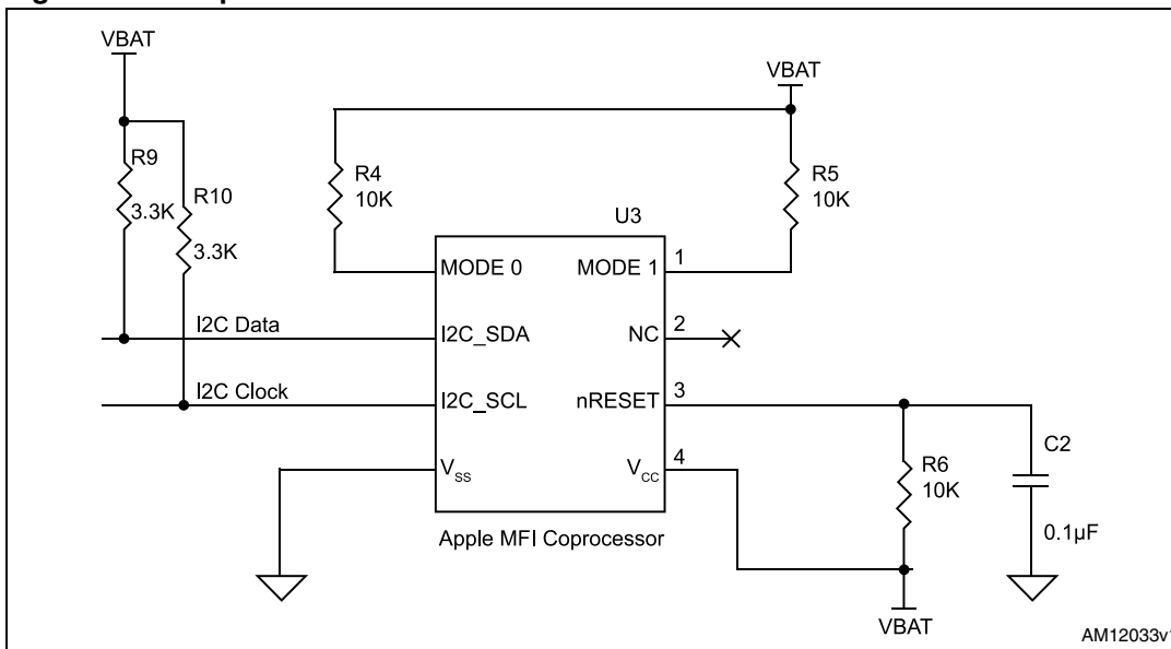
Figure 13. Co-processor
