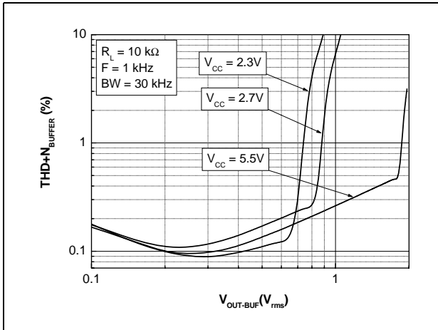
Figure 13. Output THD+N vs. output voltage ( R_L = 10k\Omega )
