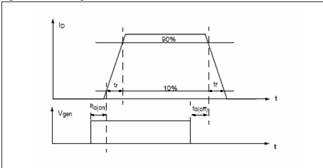
Figure 15. Switching characteristics
