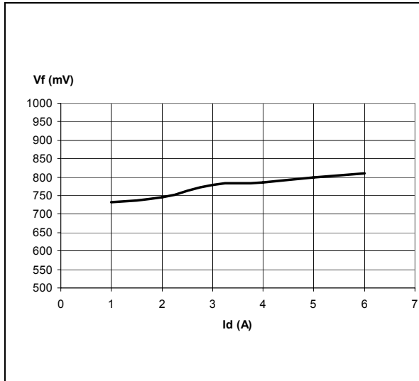
Figure 6. Source diode forward characteristics
