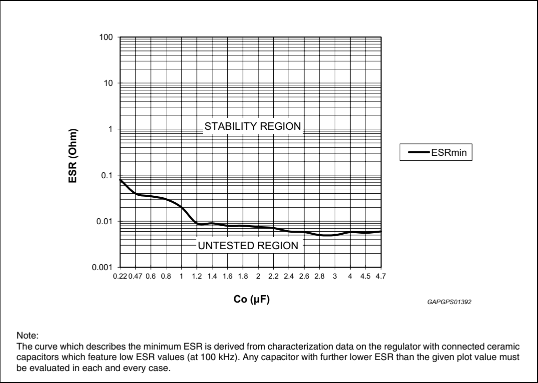
Figure 18. Stability region
