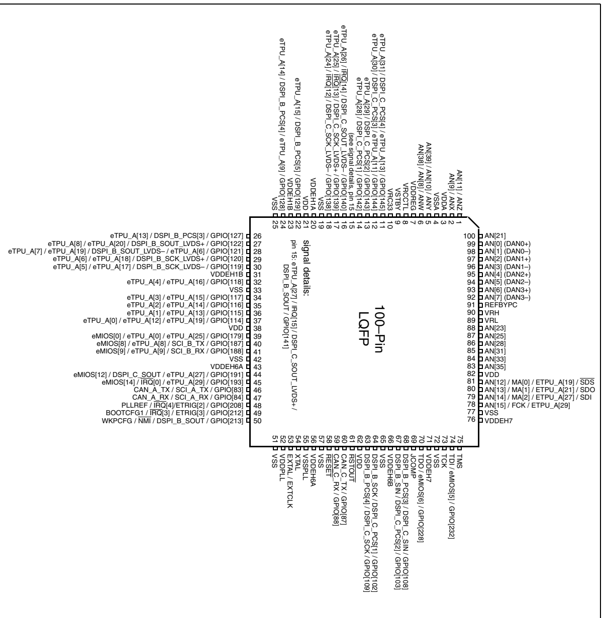
Figure 2. 100-pin LQFP pinout (top view)
