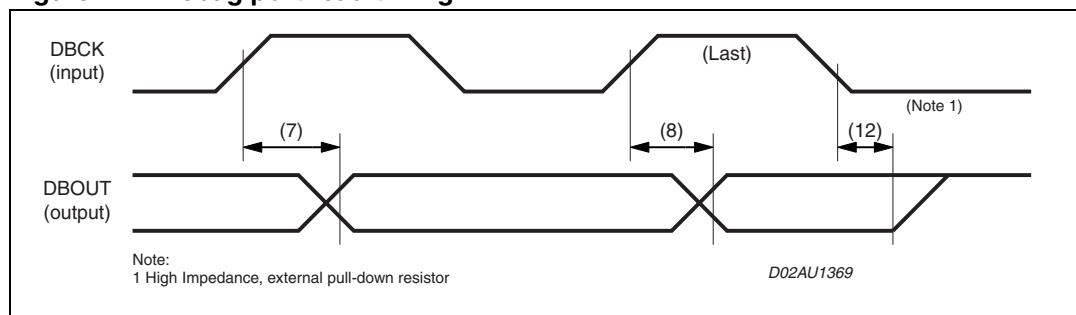
Figure 12. Debug port read timing
