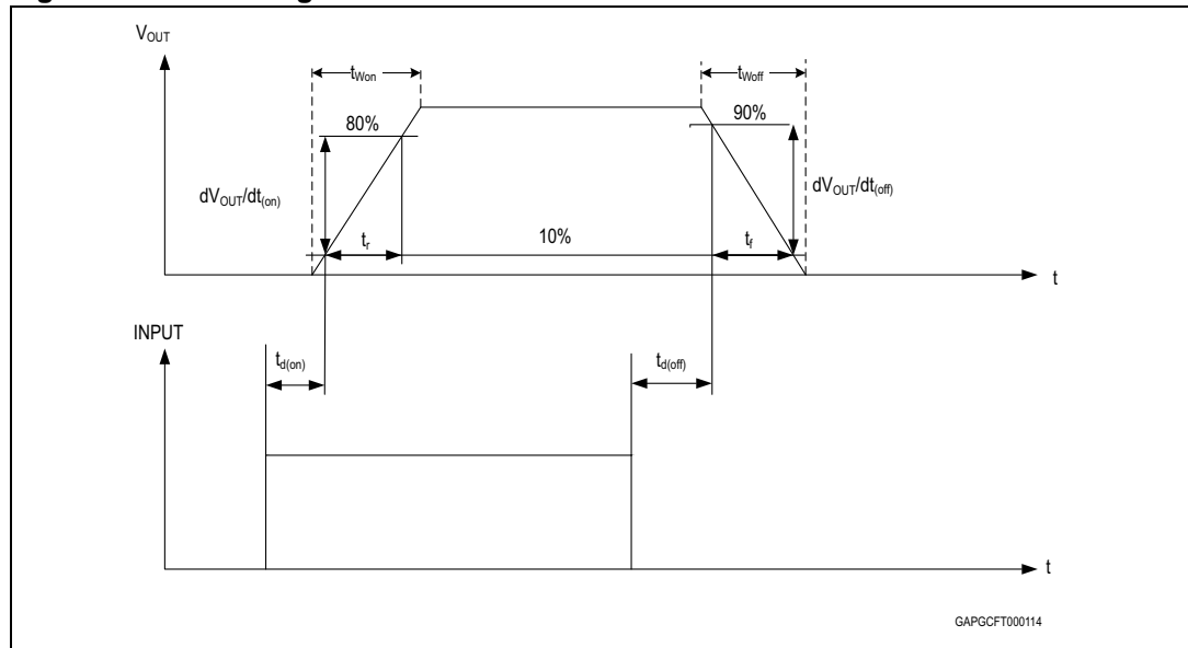
Figure 8. Switching characteristics
