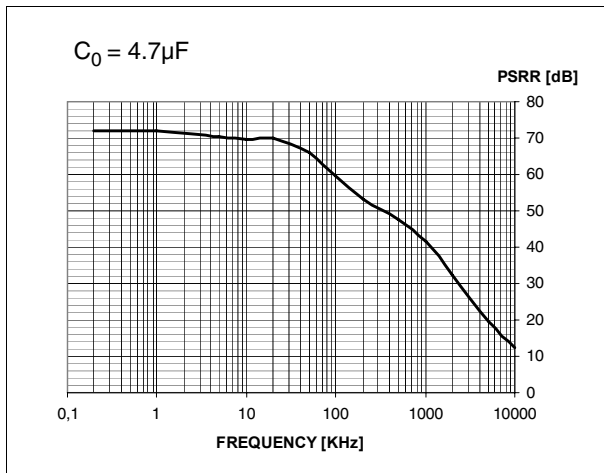
Figure 21. PSRR
