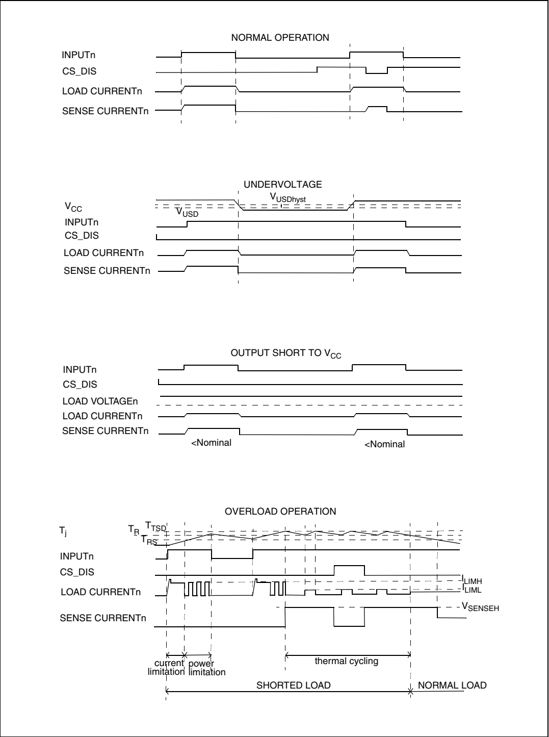
Figure 6. Waveforms
