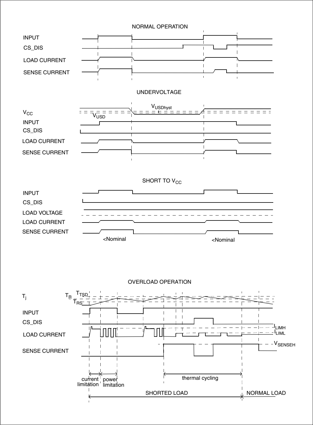
Figure 10. Waveforms
