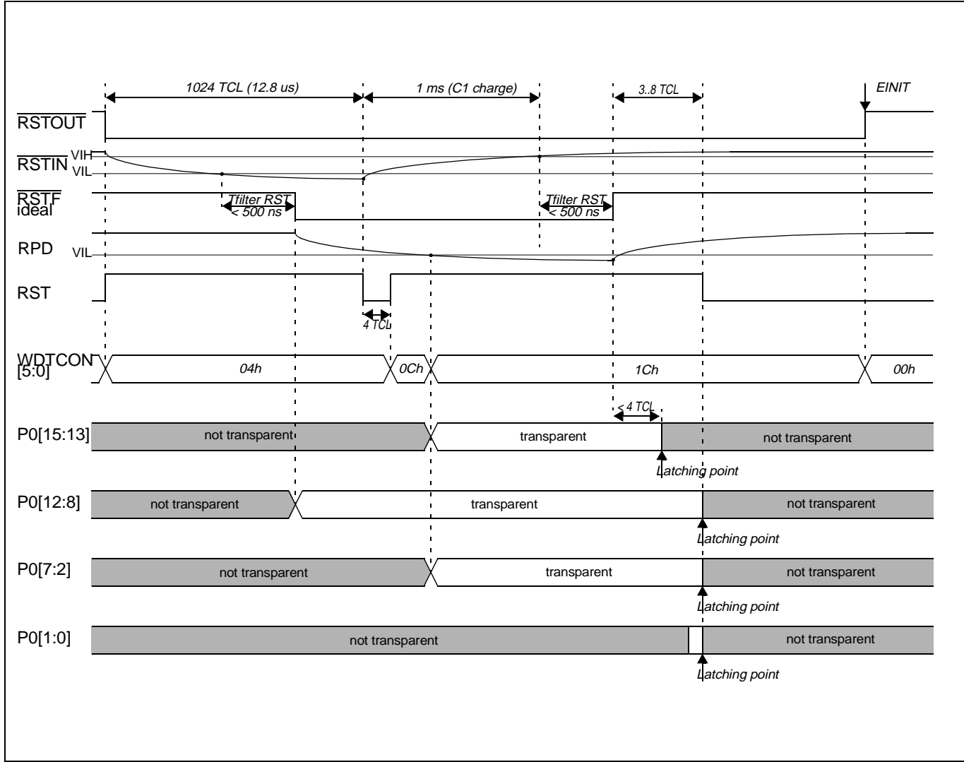
Figure 32. Example of software or watchdog bidirectional reset ( EA = 0 )
