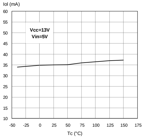
Figure 17. Openload On State Detection Threshold
