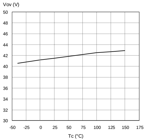
Figure 25. Overvoltage Shutdown
