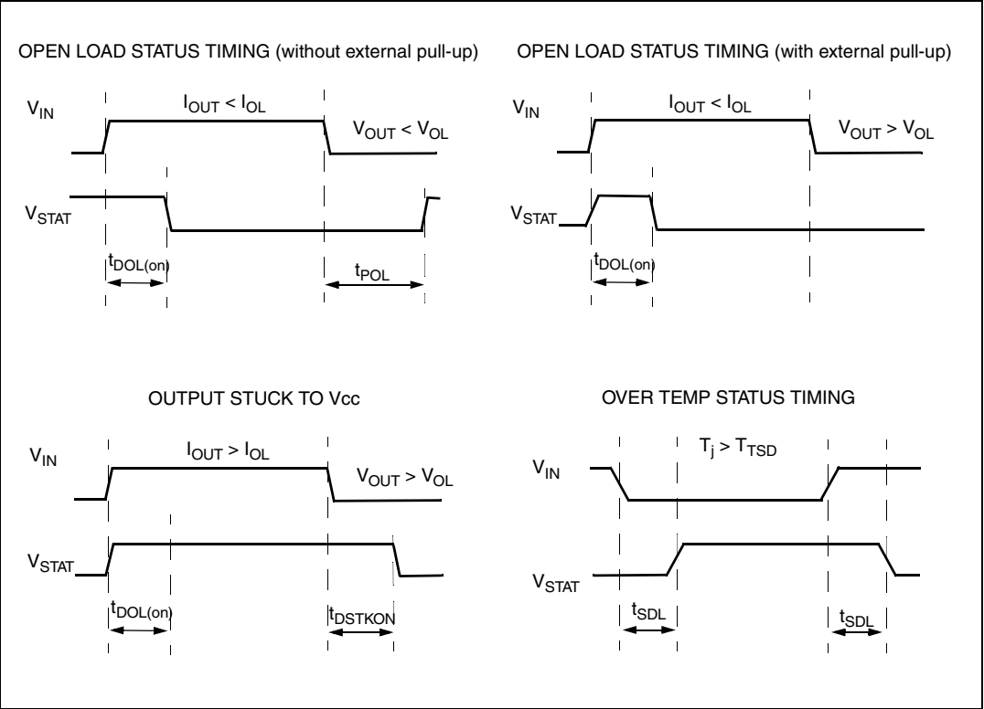
Figure 4. Status timings
