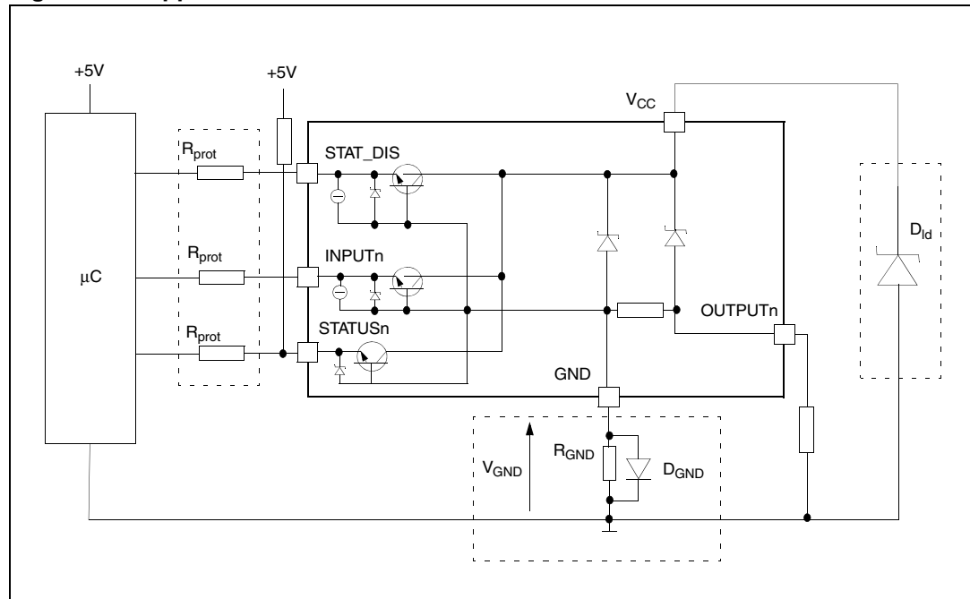
Figure 27. Application schematic
