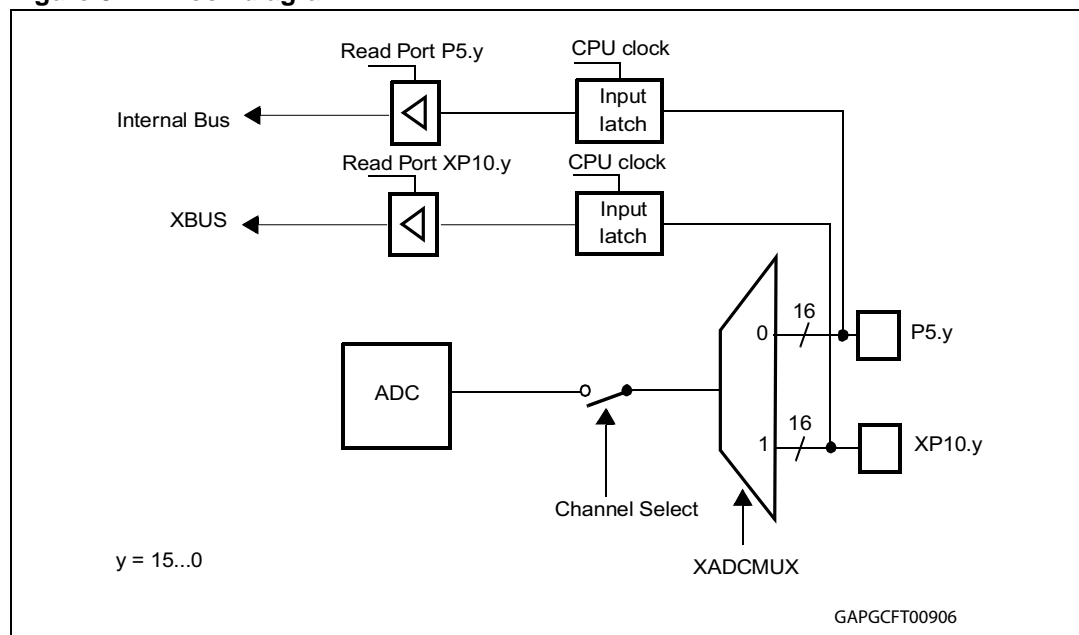
Figure 52. Block diagram
