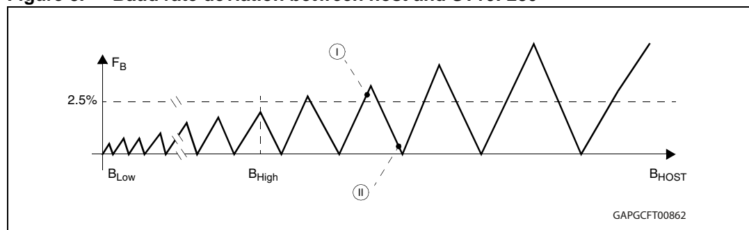
Figure 8. Baud rate deviation between host and ST10F280
