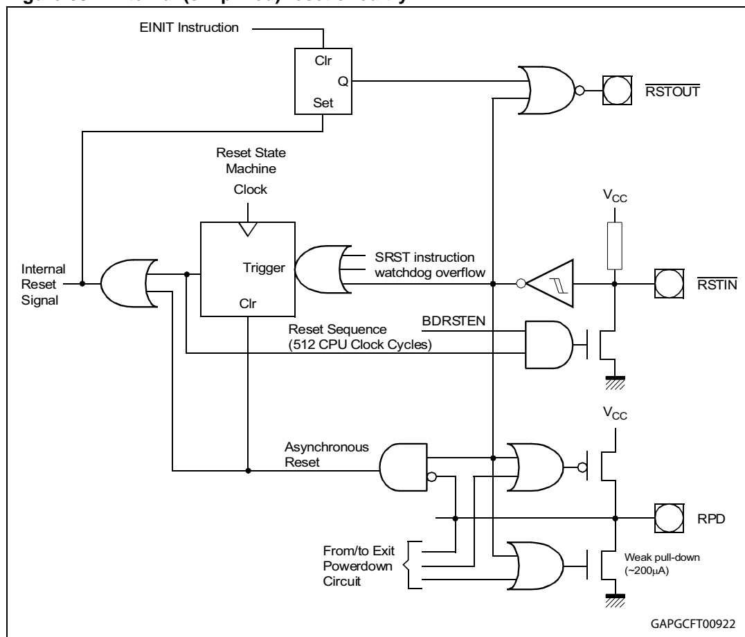
Figure 68. Internal (simplified) reset circuitry
