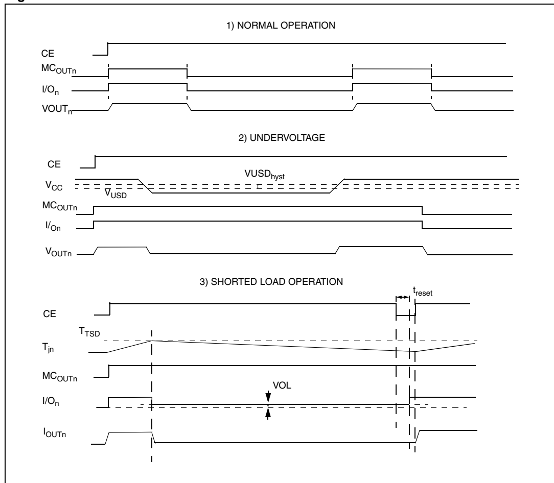
Figure 6. Waveforms
