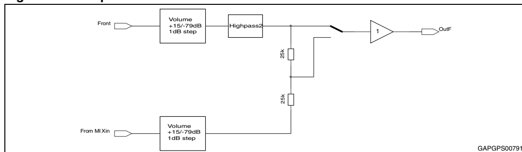
Figure 18. Output selector
