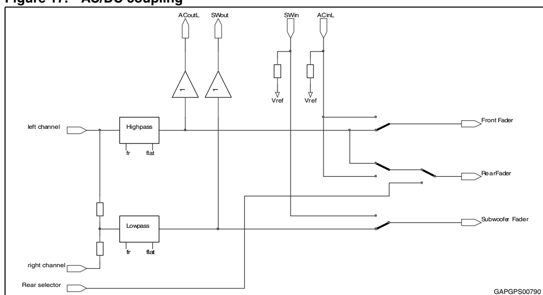
Figure 17. AC/DC coupling
