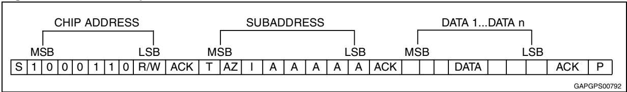
Figure 20. Interface protocol
