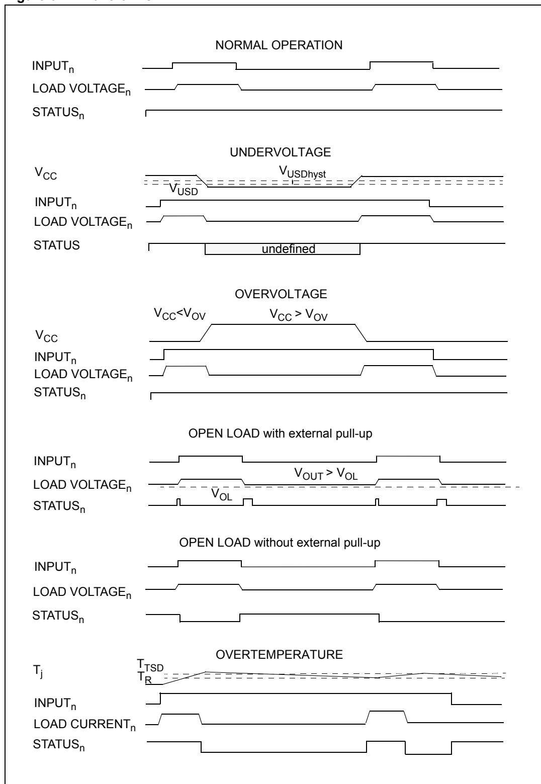
Figure 6. Waveforms
