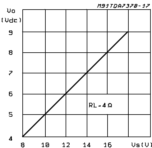
Figure 2: Quiescent Output Voltage vs. Supply Voltage (Bridge/Single Ended)
