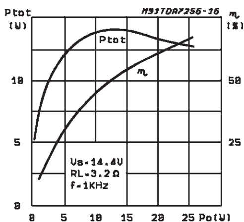
Figure 15: Power Dissipation &amp; Efficiency vs. Output Power
