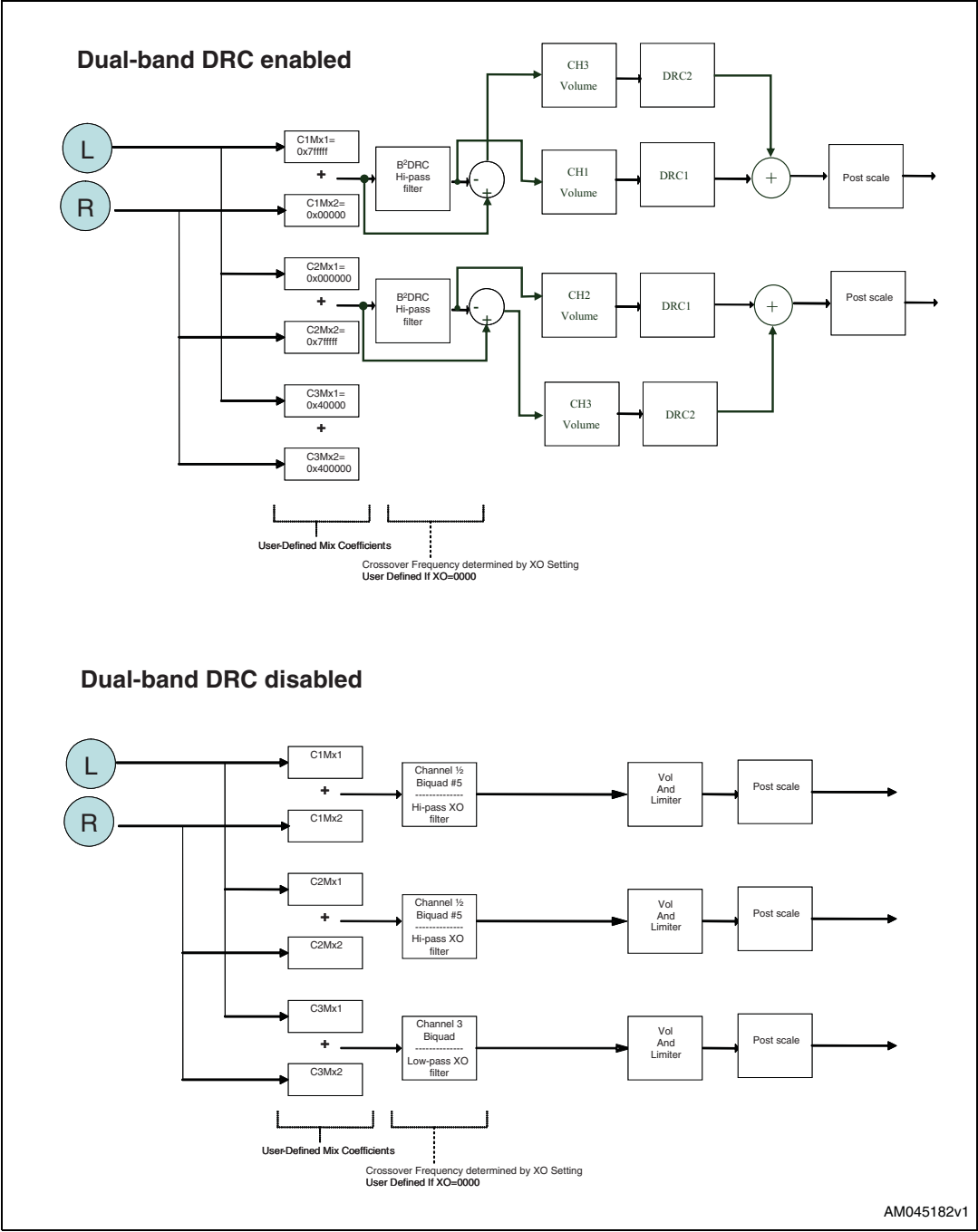
Figure 17. Processing - part 2
