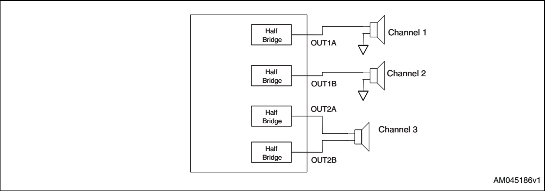
Figure 22. OCFG = 10
