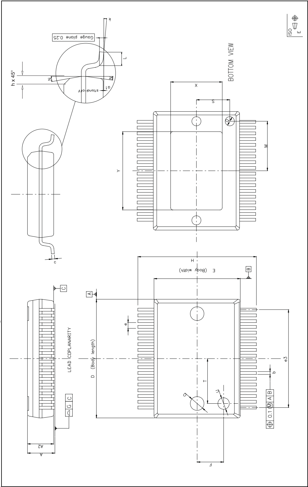
Figure 37. PowerSSO-36 EPD outline drawing
