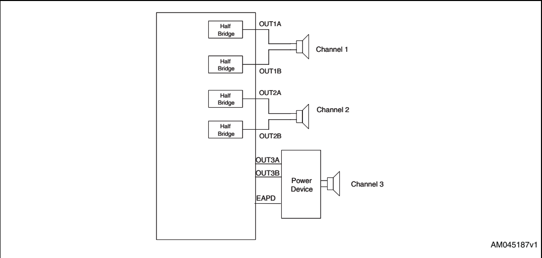
Figure 22. OCFG = 10
