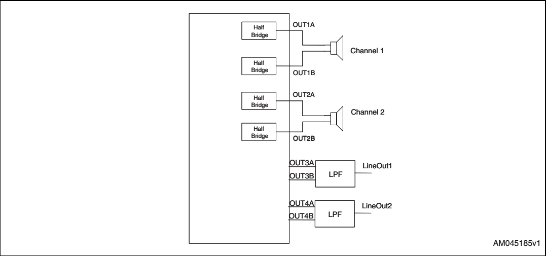
Figure 21. OCFG = 01
