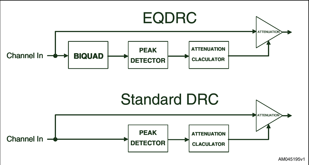
Figure 30. EQDRC scheme
