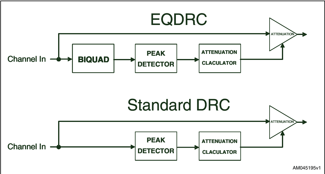
Figure 30. EQDRC scheme
