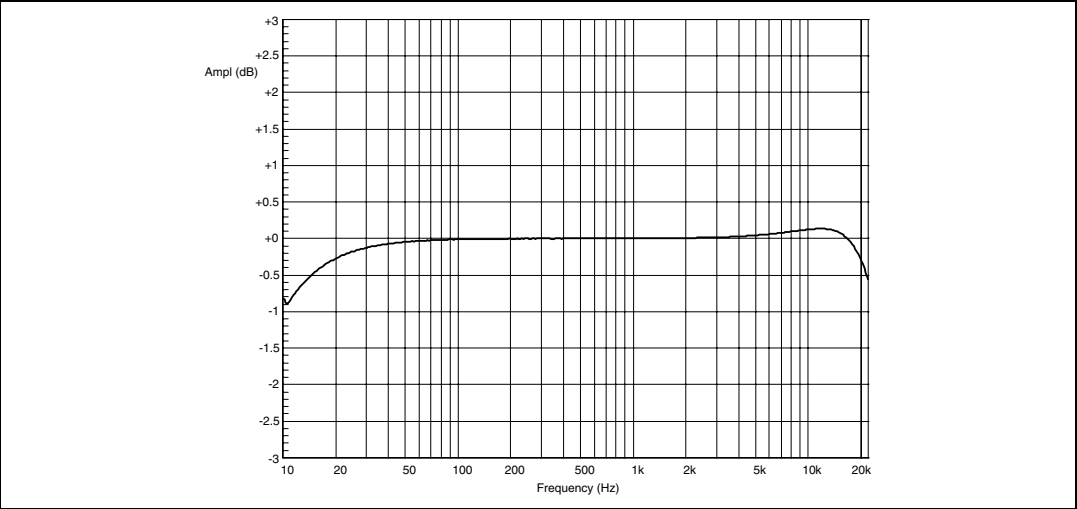
Figure 8. Frequency response
