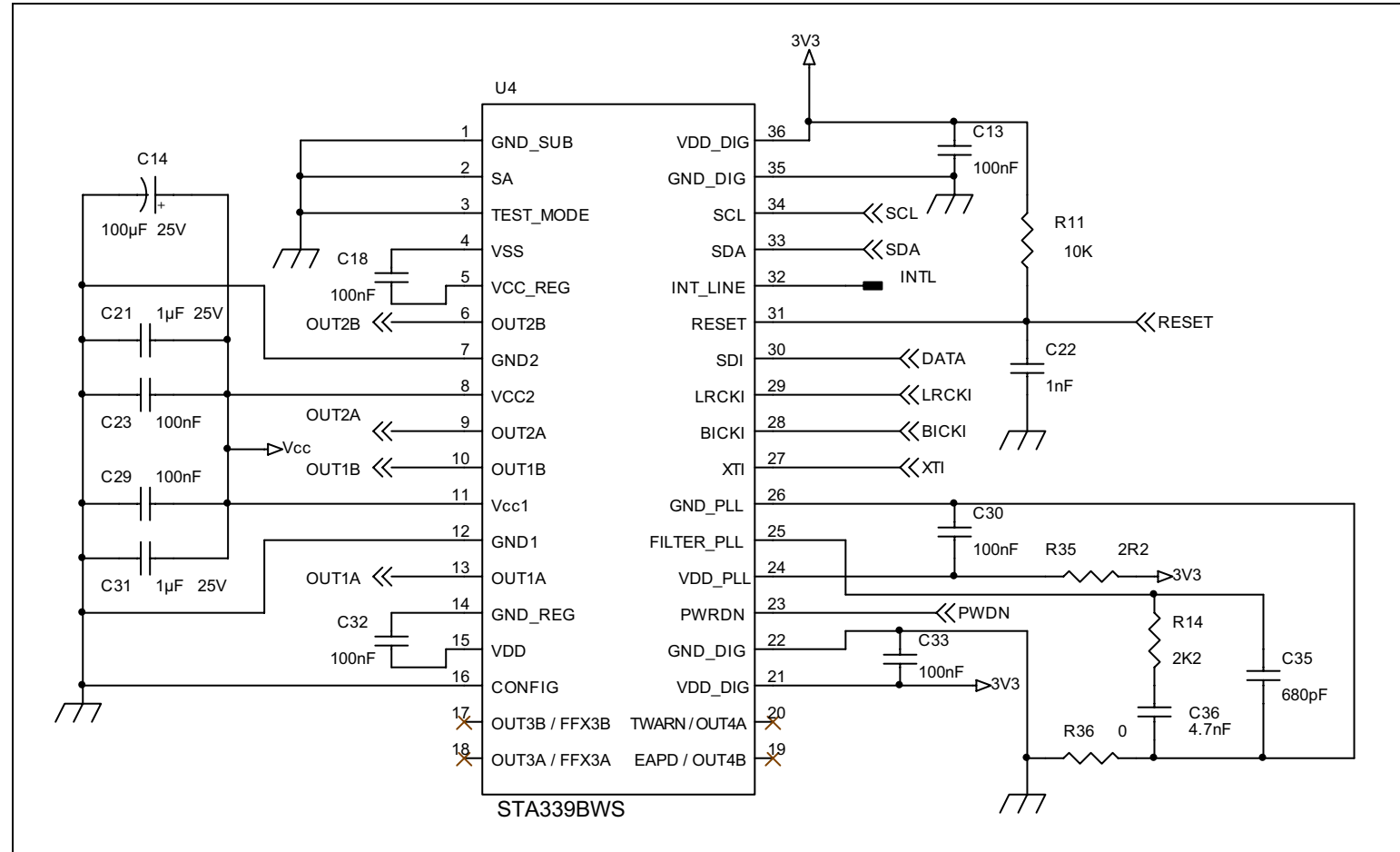
Figure 22. Applications circuit
