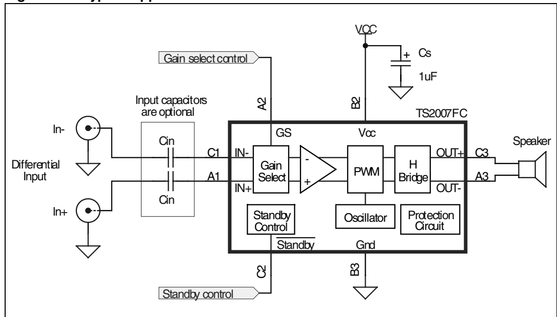
Figure 1. Typical application
