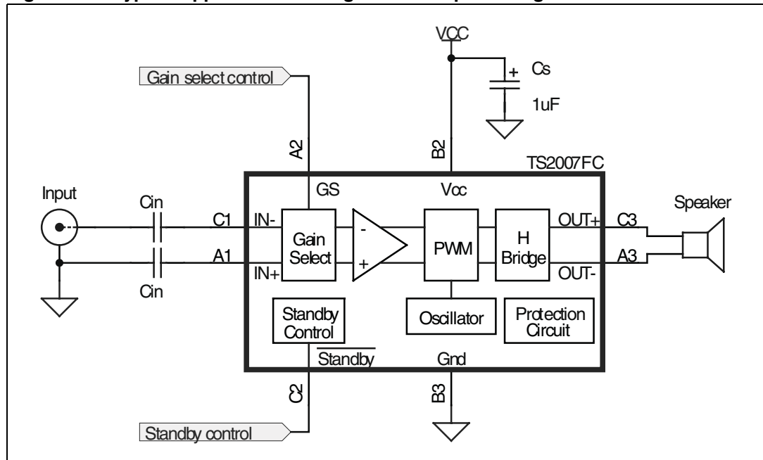
Figure 44. Typical application for single-ended input configuration
