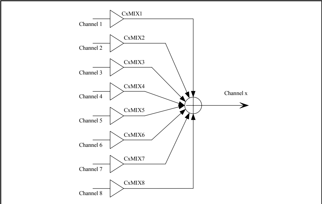
Figure 8. Channel mixer
