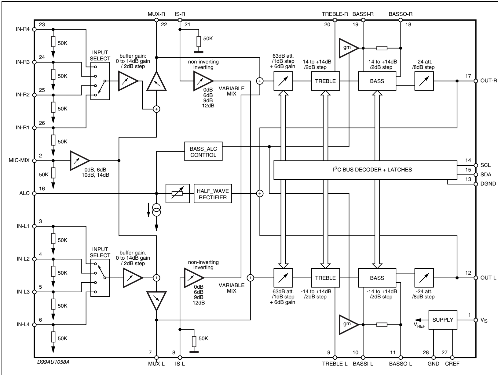
Figure 3. BLOCK DIAGRAM
