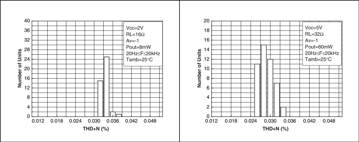
Figure 75. Best case distribution of THD + N Figure 76. Worst case distribution of THD + N
