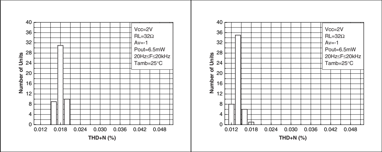
Figure 77. Typical distribution of TDH + N Figure 78. Best case distribution of THD + N
