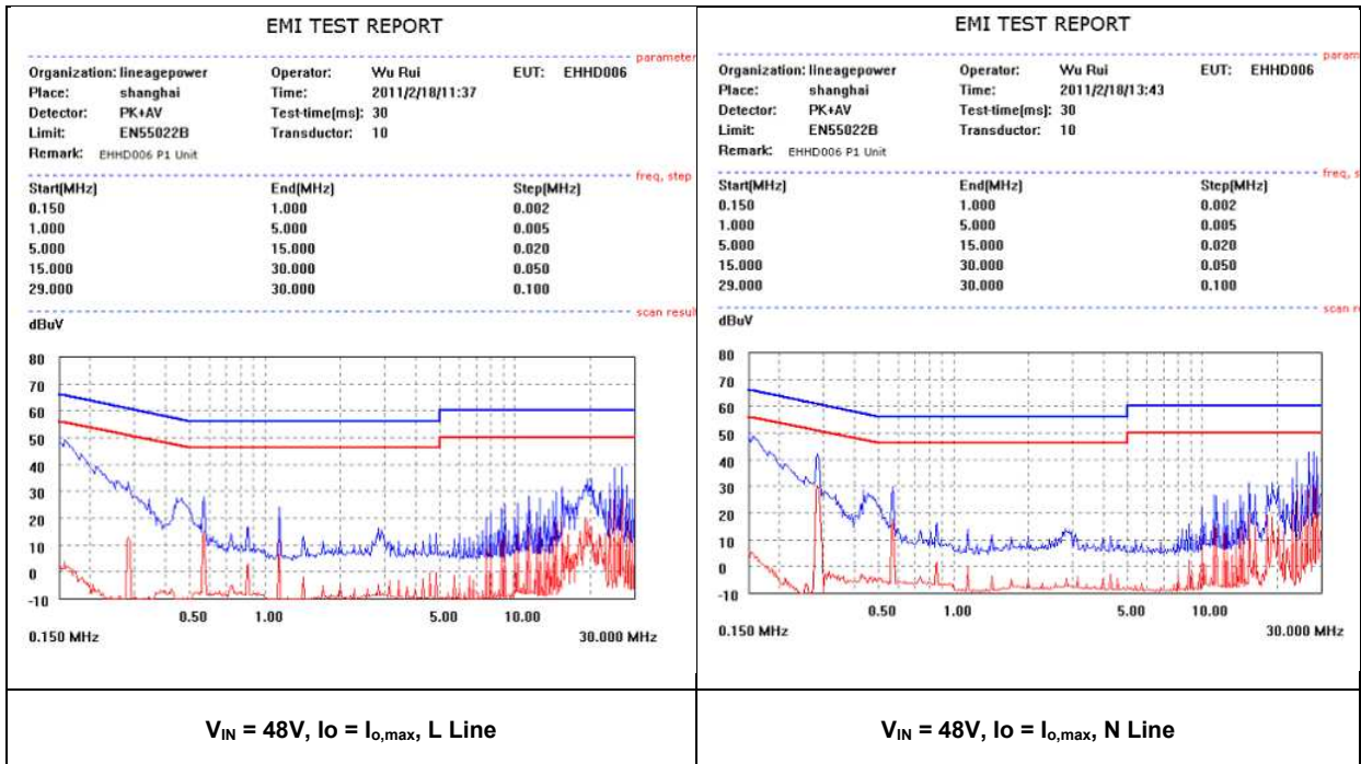
Figure 26. EMC Considerations
