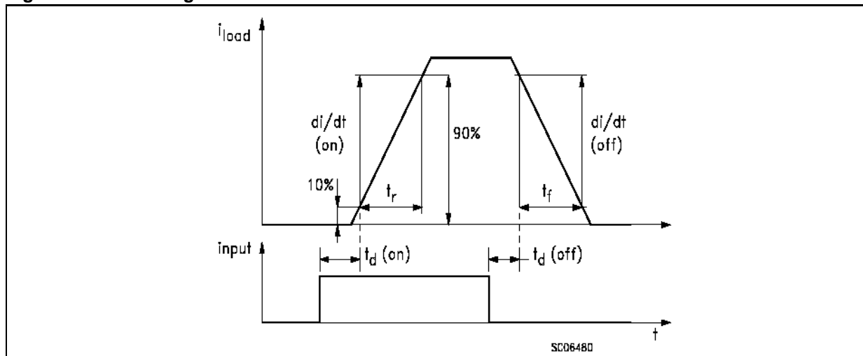
Figure 3. Switching Characteristics
