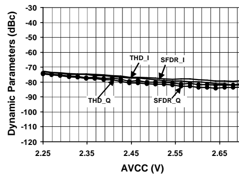
Figure 12. Distortion vs. AV_{CC} F_S=20\text{Mpsps} ; I_{CCA}=40\text{mA} ; F_{in}=5\text{MHz}
