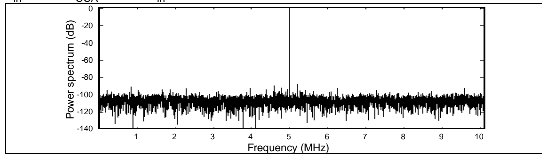
Figure 22. Dual-tone 8K FFT at 20Msps - Channel I
