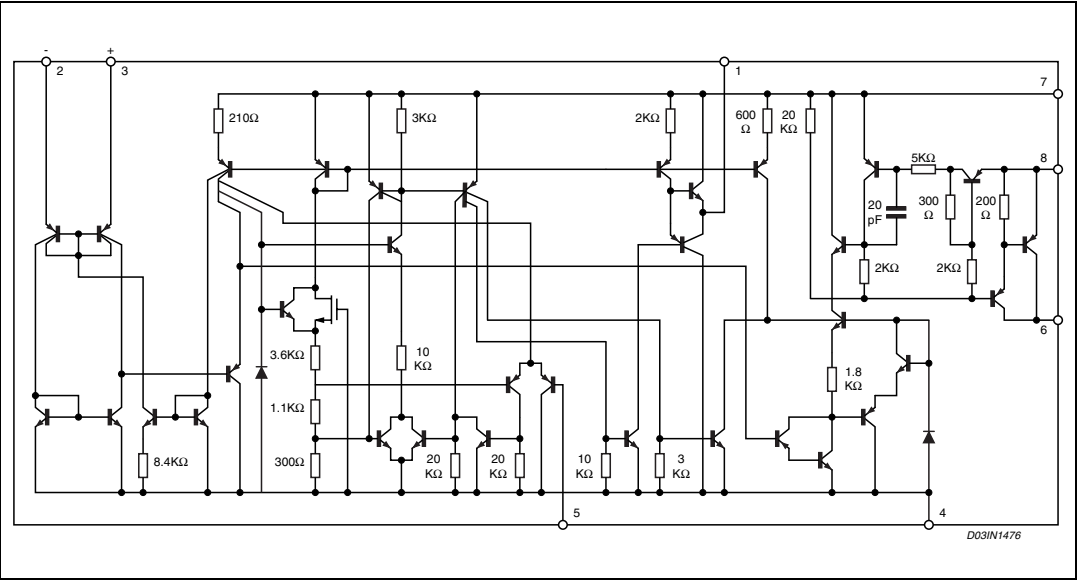
Figure 2. Schematic diagram
