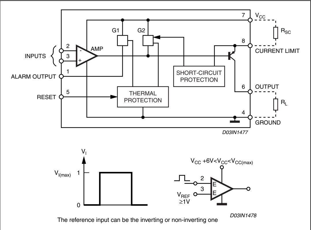
Figure 3. Equivalent schematic
