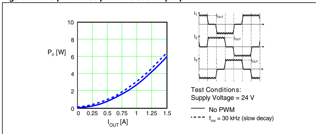
Figure 24. IC power dissipation versus output power
