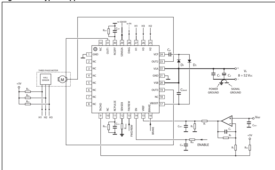
Figure 23. Typical application
