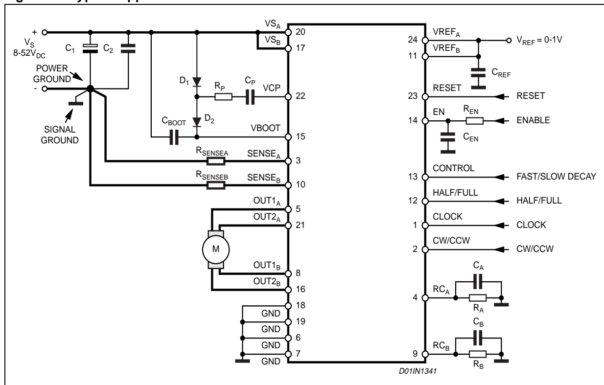
Figure 23. Typical Application
