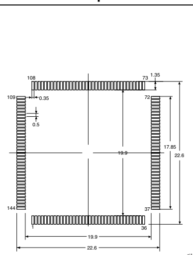
Figure 37. Recommended footprint
