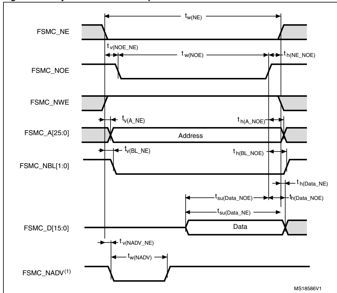
Figure 15. Asynchronous non-multiplexed SRAM/PSRAM/NOR read waveforms
