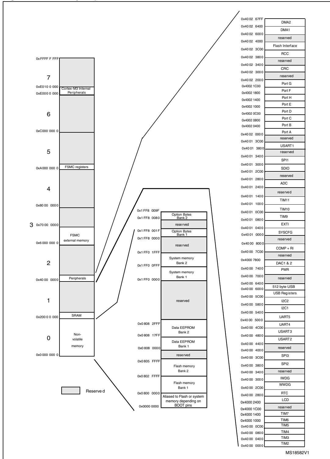
Figure 6. Memory map
