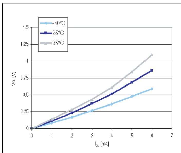
Figure 25: Typ. V_{OL} @ V_{DD} = 3.3 V (standard ports)
