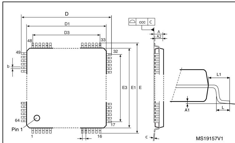
Figure 47. LQFP64 – 10 x 10 mm, 64 pin low-profile quad flat package outline (1)
