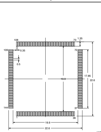
Figure 63. Recommended footprint (1)(2)
