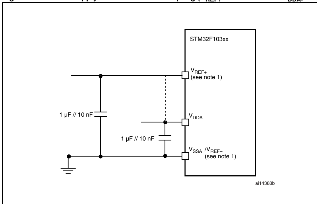
Figure 57. Power supply and reference decoupling ( V_{\text{REF}+} not connected to V_{\text{DDA}} )
