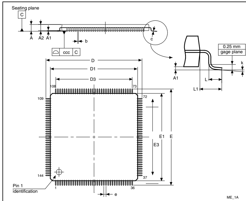
Figure 54. LQFP144, 20 x 20 mm, 144-pin thin quad flat package outline (1)
