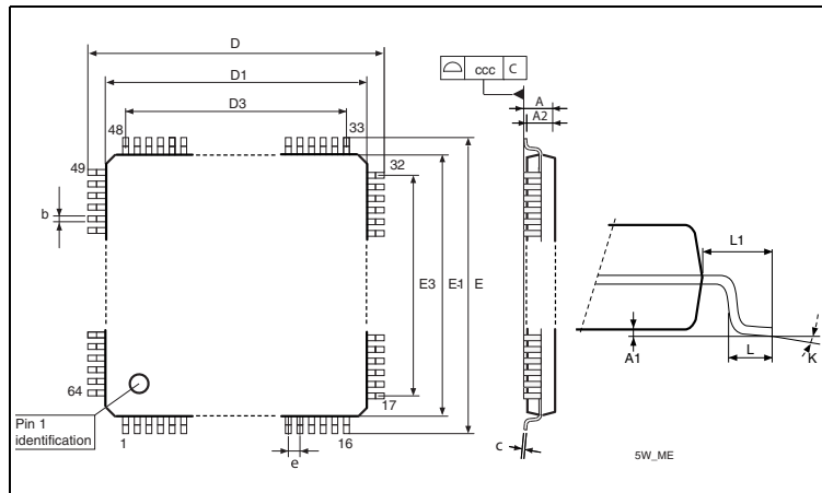
Figure 58. LQFP64 – 10 x 10 mm, 64 pin low-profile quad flat package outline (1)
