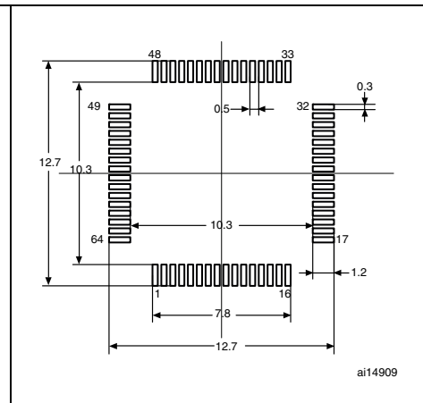
Figure 59. Recommended footprint (1)(2)
