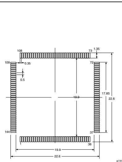
Figure 55. Recommended footprint (1)(2)
