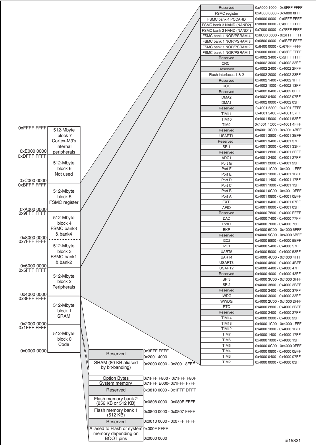
Figure 6. Memory map
