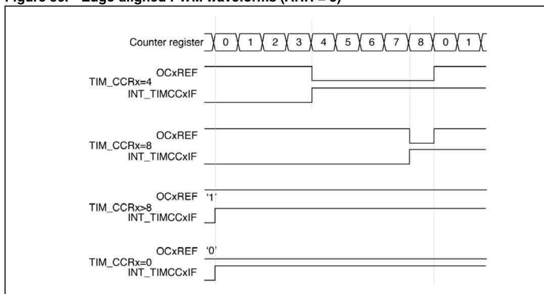
Figure 36. Edge-aligned PWM waveforms (ARR = 8)
