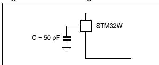
Figure 54. Pin loading conditions
