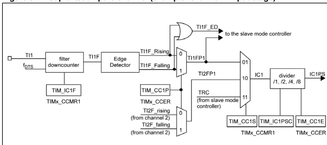
Figure 31. Capture/compare channel (example: channel 1 input stage)
