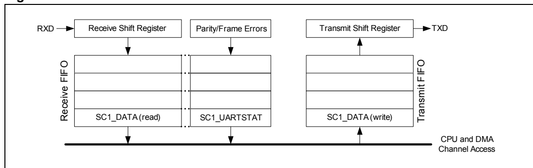
Figure 13. UART FIFOs
