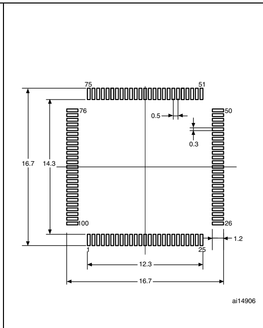
Figure 79. Recommended footprint (1)(2)
