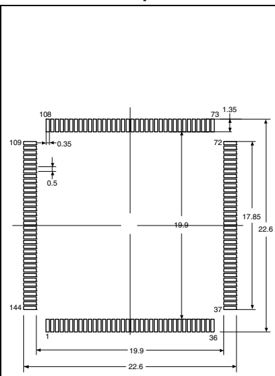
Figure 81. Recommended footprint (1)(2)
