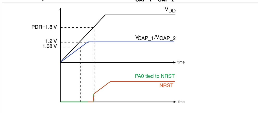
Figure 7. Startup in regulator OFF: slow V_{DD} slope - power-down reset risen after V_{CAP\_1}/V_{CAP\_2} stabilization
