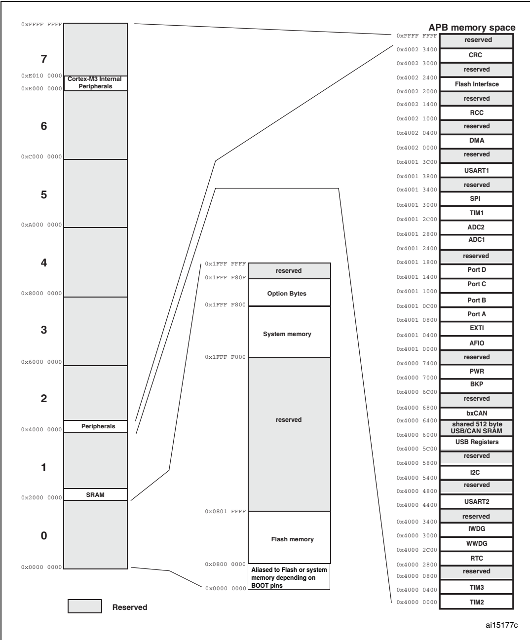
Figure 8. Memory map
