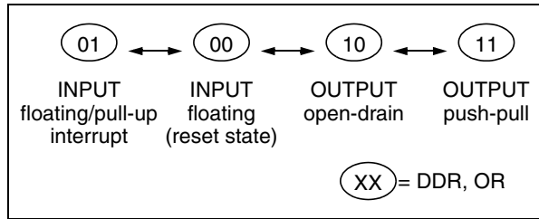
Figure 21. Interrupt I/O Port State Transitions
