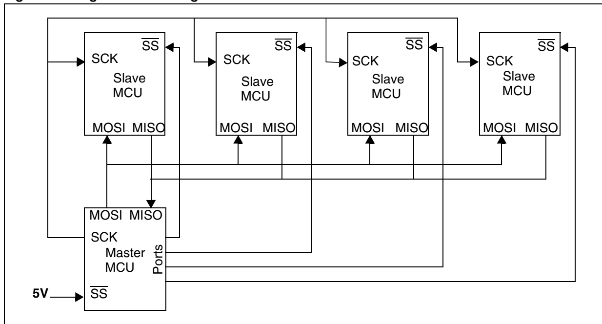
Figure 46. Single Master Configuration
