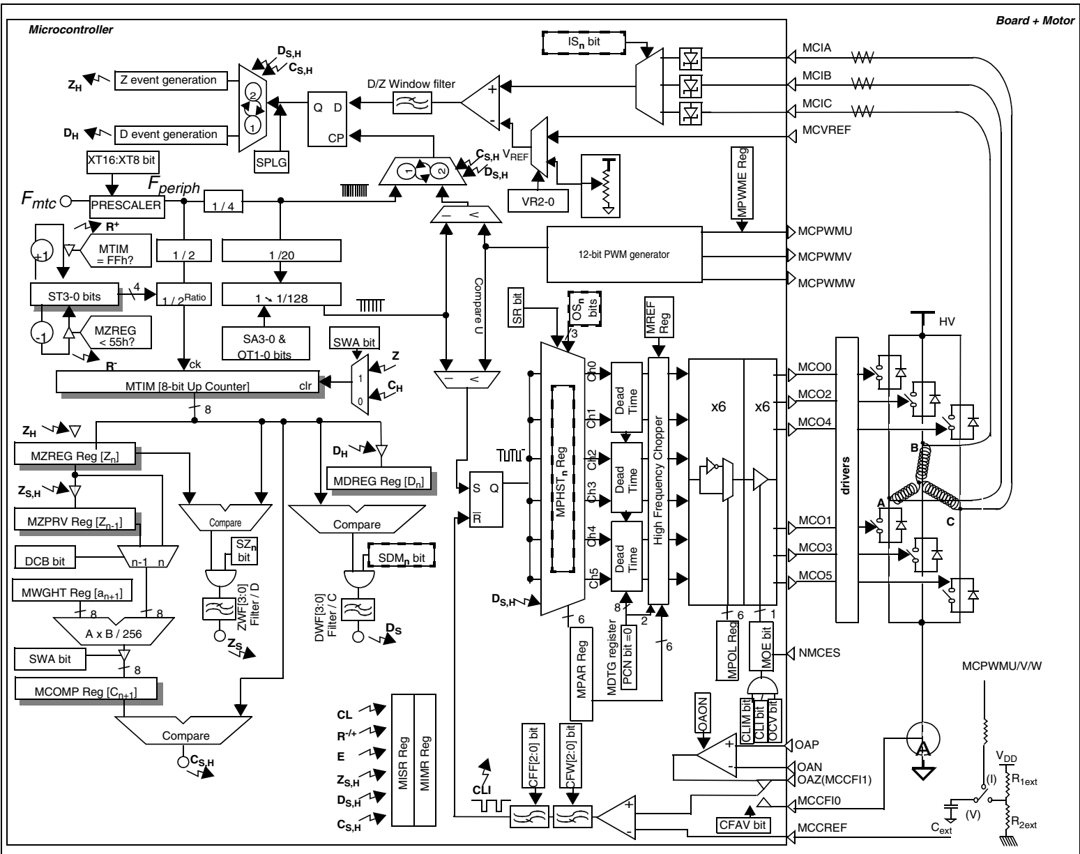
Figure 123. General view of the MTC for PM BLDC motor control
