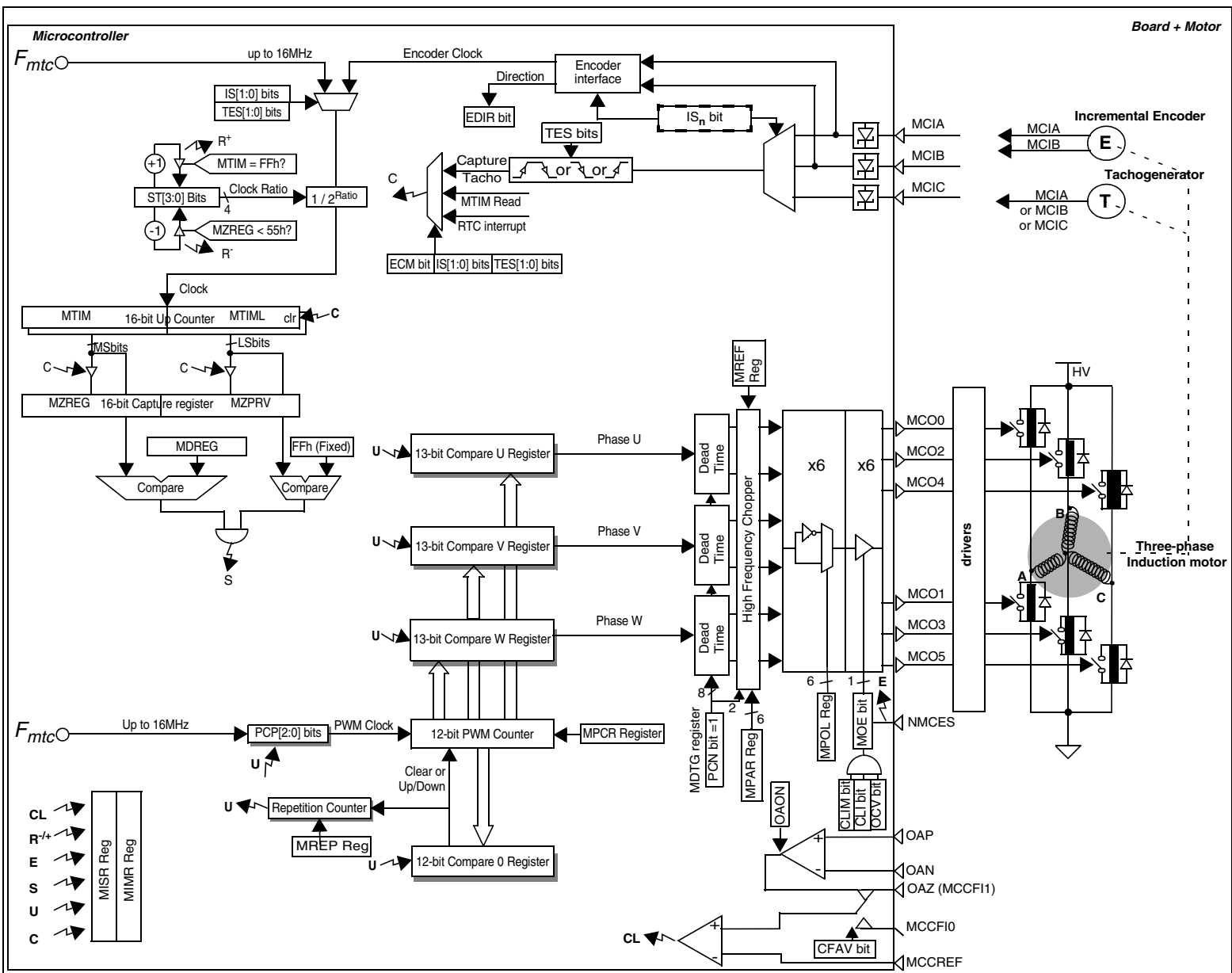
Figure 124. General view of the MTC configured for Induction motor control (proposal)
