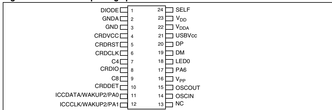
Figure 3. 24-Pin SO package pinout
