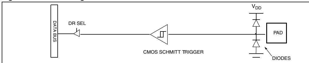
Figure 24. PA6 configuration
