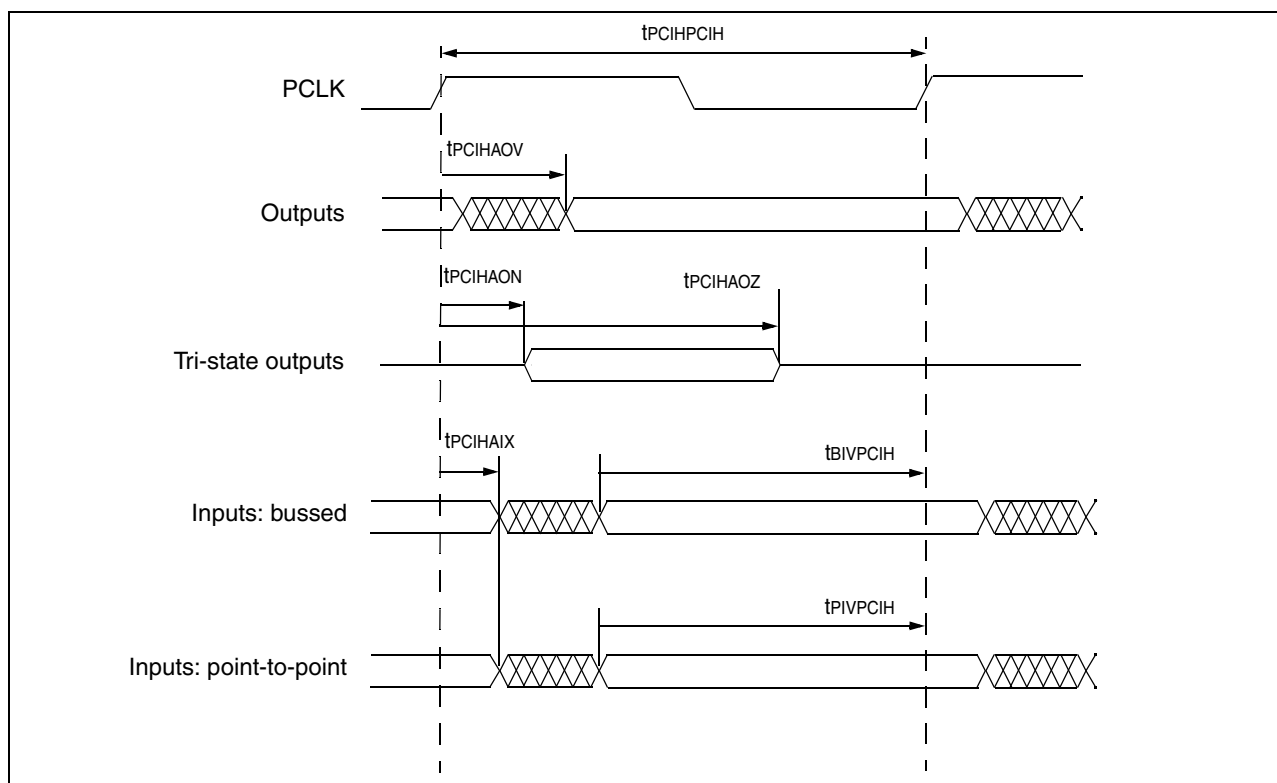
Figure 11: PCI timings
