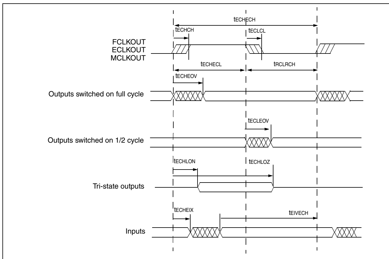
Figure 15: EMI AC timings
